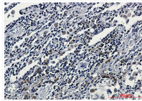
ATF6 antibody immunohistochemistry human lung cancer STJA0035123
