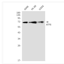
ATF6 antibody western blot A549 HL-60 U2OS STJA0035123
