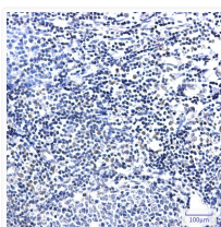
PIM1 antibody immunohistochemistry human tonsil STJA0035030
