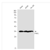
PIM1 antibody western blot HeLa A549 HL-60 STJA0035030
