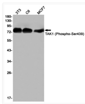
Phospho-TAK1 Ser439 antibody western blot 3T3 C6 MCF-7 STJA0034910
