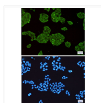
STUB1 antibody western blot K562 rat brain C6 3T3 HeLa STJA0034897
