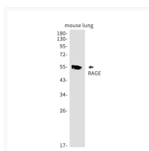
RAGE antibody western blot mouse lung lysates STJA0034792
