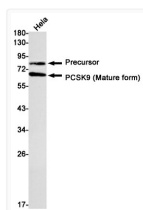
PCSK9 antibody western blot HeLa lysates STJA0034697
