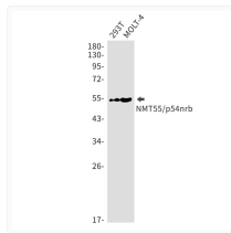
NONO antibody western blot NMT55/p54nrb 293T MOLT4 STJA0034646
