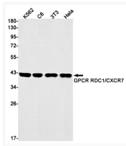
RDC1 antibody western blot K562 C6 3T3 HeLa STJA0034386
