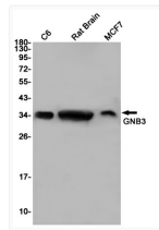
GNB3 antibody western blot C6 rat brain MCF-7 STJA0034383
