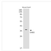
GNB3 antibody western blot mouse heart STJA0034383
