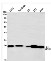
eIF4E antibody western blot K562 rat brain C6 3T3 HeLa STJA0034271
