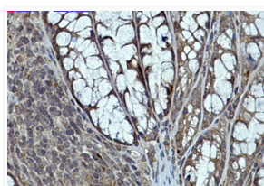
eIF4E antibody immunohistochemistry mouse colon STJA0034271
