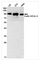
CUL5 antibody western blot C6 3T3 HeLa STJA0034211
