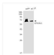
ATG16L1 antibody western blot HeLa PC-12 STJA0034049
