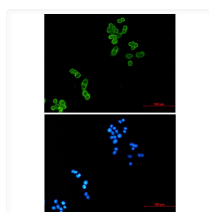
Thioredoxin antibody immunocytochemistry HeLa cells STJA0033842
