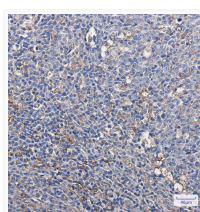
Thioredoxin/TRX antibody immunohistochemistry human tonsil STJA0033842
