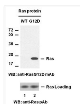
Ras G12D antibody western blot recombinant proteins STJA0033656
