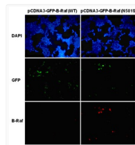
B-Raf antibody immunofluorescence HEK293T cells STJA0033562
