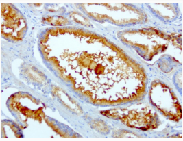
Syntenin 1 antibody immunohistochemistry human prostate cancer STJA0033331
