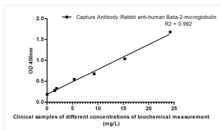
Beta2-microglobulin antibody sandwich ELISA standard curve STJA0033236
