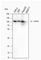
GRP94 antibody western blot HeLa 293 HepG2 MCF-7 STJA0033094
