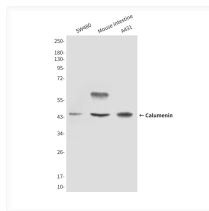
Calumenin antibody western blot SW480 mouse intestine A431 STJA0032407
