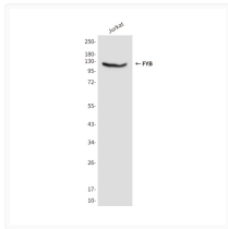
FYB antibody western blot Jurkat lysates STJA0032404
