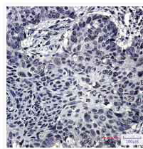
SRSF3 antibody immunohistochemistry human lung cancer STJA0012690
