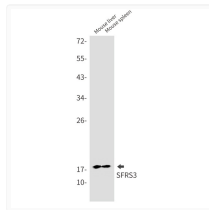
SRSF3 antibody western blot mouse liver spleen STJA0012690
