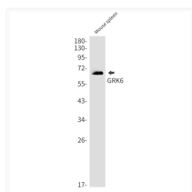
Western blot analysis of GRK6 in mouse spleen lysates using GRK6 antibody.
