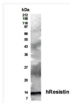
Western Blot specific immunolabeling Resistin in transfected 293 cell lysate STJA0005715
