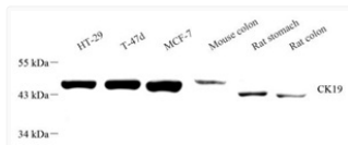
Western blot analysis of CK19 at dilution of 1:1000
