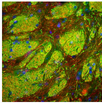
IHC staining with CNP in mouse striatum myelinating oligodendrocytes STJA0004898
