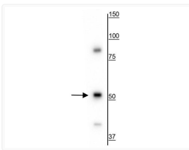
Western blot analysis detecting 50 kDa vimentin protein in HeLa cell lysate STJA0003872
