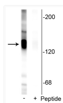
Western blot KCC2 phospho-Ser940 labeling in rat hippocampal lysate STJA0003753
