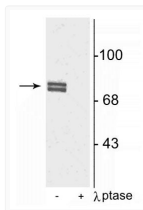
Western blot 5-LO Ser523 phosphorylation in rat cortical lysate with phosphatase control STJA0003568
