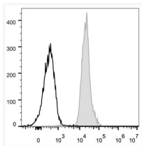
C57BL/6 murine splenocytes were stained with Anti-CD48 antibody (STJA0000222) [Used at 0.2 \mu g/ 10^6 cells dilution] (filled gray histogram). Unstained lymphocytes (empty black histogram) were used as control.
