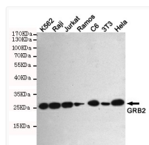
Western blot detection of GRB2 in K562, Raji, Jurkat, Ramos, C6, 3T3 and HeLa cell lysates using GRB2 mouse mAb (1:1000 diluted). Predicted band size: 25KDa. Observed band size: 25KDa.
