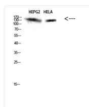
Western blot analysis of HEPG2, HELA cells using Antibody diluted at 500. Secondary antibody was diluted at 1:20000
