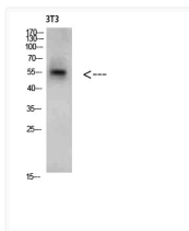
Western blot analysis of 3T3 cells using CREB3 Polyclonal Antibody diluted at 1:2000. Secondary antibody was diluted at 1:20000
