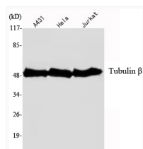
Western blot analysis using Tubulin Beta monoclonal antibody against A431, HeLa, Jurkat cell lysate.
