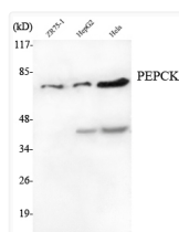
Western blot analysis using PEPCK monoclonal antibody against ZR75-1, HepG2, HeLa cell lysate.
