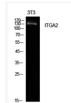
Western blot analysis of NIH-3T3 cells using Integrin Alpha 2 Polyclonal Antibody.. Secondary antibody was diluted at 1:20000
