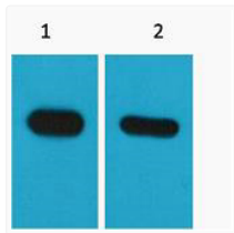
Western blot analysis of CBP recombinant protein, diluted at, 1) 1:5000 , 2) 1:10000
