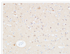
Immunohistochemical analysis of paraffin-embedded Human Cerebral cortex. 1, Antibody was diluted at 1:200 (4°C overnight). 2, High-pressure and temperature EDTA, pH8.0 was used for antigen retrieval. 3, Secondary antibody was diluted at 1:200 (room temperature, 30min).
