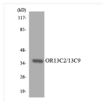
Western blot analysis of the lysates from K562 cells using OR13C2/13C9 antibody.
