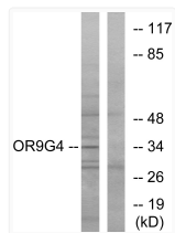
Western blot analysis of lysates from HeLa cells, using OR9G4 Antibody. The lane on the right is blocked with the synthesized peptide.
