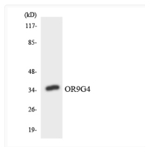
Western blot analysis of the lysates from HeLa cells using OR9G4 antibody.
