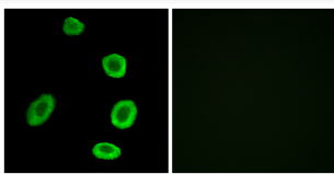
Immunofluorescence analysis of A549 cells, using OR8K1 Antibody. The picture on the right is blocked with the synthesized peptide.
