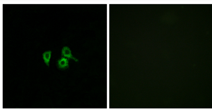
Immunofluorescence analysis of A549 cells, using OR10H4 Antibody. The picture on the right is blocked with the synthesized peptide.
