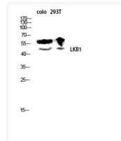
Western blot analysis of colo 293T lysis using LKB1 antibody. Antibody was diluted at 1:500
