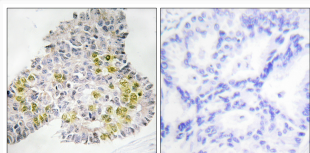
Immunohistochemistry analysis of paraffin-embedded human lung carcinoma tissue, using LKB1 Antibody. The picture on the right is blocked with the synthesized peptide.
