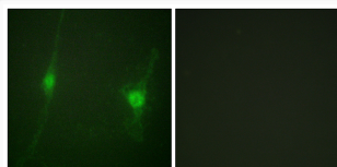
Immunofluorescence analysis of NIH/3T3 cells, using LKB1 Antibody. The picture on the right is blocked with the synthesized peptide.
