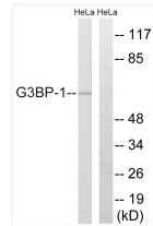
Western blot analysis of lysates from HeLa cells, using G3BP-1 Antibody. The lane on the right is blocked with the synthesized peptide.
