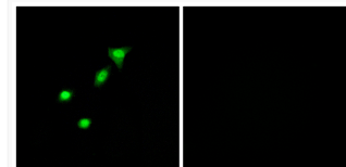
Immunofluorescence analysis of A549 cells, using REQU Antibody. The picture on the right is blocked with the synthesized peptide.
