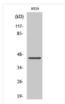
Western blot analysis of various cells using DPF2 Polyclonal Antibody
