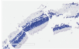
STJ73560 Negative Control showing staining of paraffin embedded Human Retina, with no primary antibody.
