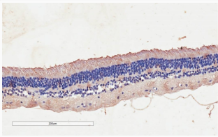
STJ73560 (2µg/ml) staining of paraffin embedded Human Retina. Microwaved antigen retrieval with citrate buffer pH 6, HRP-staining.
