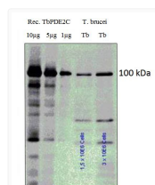
Western blot with Anti-PDE2C / PDEB1 Antibody (STJ503215) on recombinant TbPDE2C and cell extracts. Antibody at 1:1000 dilution in buffer.
