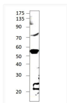
Western blot with Anti-PRKN Antibody (STJ502119) on SKNMC cell at 1:500 dilution in buffer.
