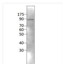
Western blot with Anti-Neurochondrin Antibody (STJ501948) with NORB peptide. Antibody at 1:500 dilution in buffer.
