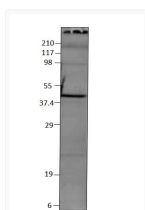
Western blot with Anti-FtsZ Antibody (STJ501091) with peptide on at 1:500 dilution in buffer.
