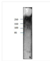
Western blot with Anti-PIEZO1 Antibody (STJ500987) with peptide on at 1:500 dilution in buffer.
